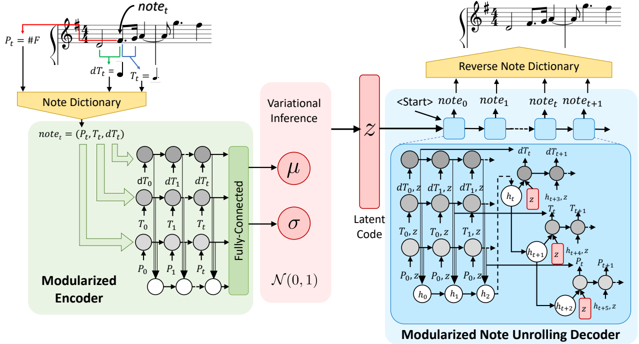
Fig. 1. The illustration of the proposed modularized framework, where the VAE architecture is embedded with a modularized encoder and a note-unrolling decoder, and the note event representations are realized by a note dictionary and a reverse note dictionary.
