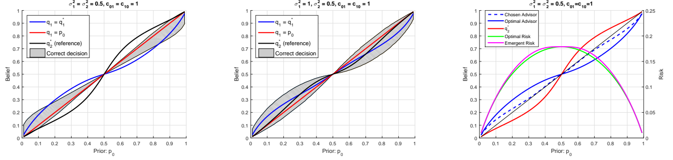
(a) Advisor selection under equal expertise. The optimal learner fails to recognize the optimal advisor and makes mistakes often.
