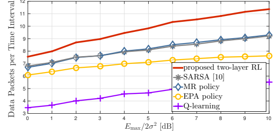
Fig. 2: Average throughput vs. E_{\max}/(2\sigma^2) .
