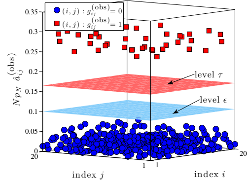
Fig. 1. A pictorial illustration of Theorem 2: the scaled estimated entries \hat{a}_{ij}^{(\text{obs})} cluster in two groups depending on whether agents i and j are interacting or not.
