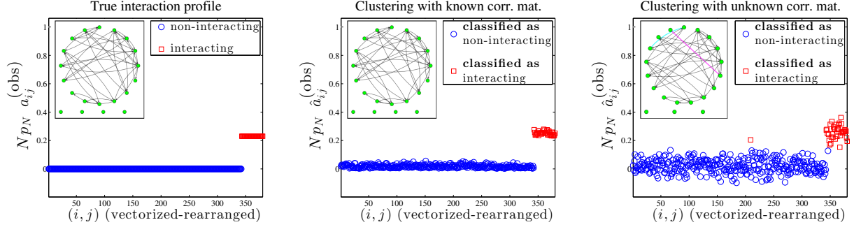
Fig. 2. Network tomography for the case of a Laplacian combination rule in (12), with parameter \lambda = 0.5 . The network size is N = 100 , where only K = 20 agents are observable. The interaction probability is p_N = 2(\ln N)/N \approx 0.092 , and the step-size is \mu = 0.1 .
