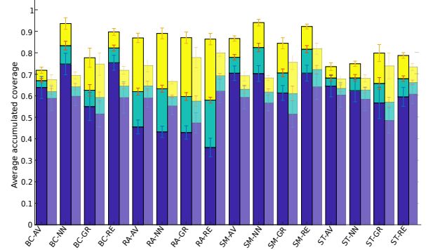
Fig. 3. Comparison of normalised accumulated coverage over all objects and the entire simulation (cp. Equation 1) for the Scenario 2 using different communication strategies (BC, RA, SM, and ST) and different response models (AV, NN, GR, and RE). The mean and standard deviation of k -coverage (blue), 2-coverage (turquoise) and 1-coverage (yellow) is shown. Results from the corresponding approaches without network-level self-awareness are shown in lightly shaded colours.
