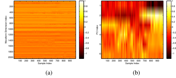
Fig. 1: Study on PCA denoising and dimension reduction. (a) Waveform series \mathbf{G}_i[l] 's before PCA. (b) Feature series \mathbf{Z}_i[l] 's after PCA.
