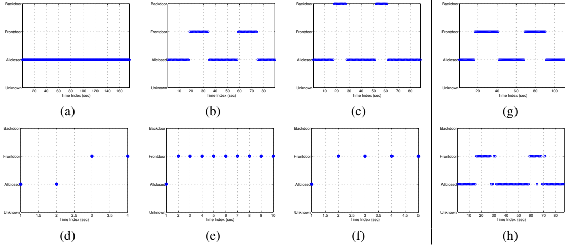
Fig. 4: Experimental results. (a)Accuracy test: 3 minutes under “all-doors-closed” with someone walking outside and close to front and back door. (b) Accuracy test: front door is opened and closed twice from outside. (c)Accuracy test: back door is opened twice from outside. (d) Robustness test: front door is opened under a fast speed. (e) Robustness test: front door is opened under a slow speed. (f) Robustness test: front door is opened to half-open. (g) Front door opened at Day 2. (h) Front door opened at Day 9.
