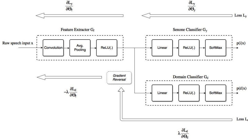
Fig. 1. The feature extractor extracts discriminative features directly from raw speech. It consists of several stages of convolution/pooling/ReLU. Senone classifier along with the feature extractor forms a standard architecture. Domain classifier is also connected to feature extractor through a gradient reversal. Reversal of gradient force the feature extractor to learn domain invariant features.
