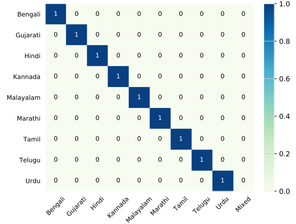
(b) Encoder-conditioned
