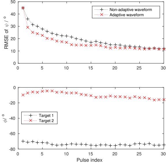
Fig. 1. RMSE and target motion for scenario 1
