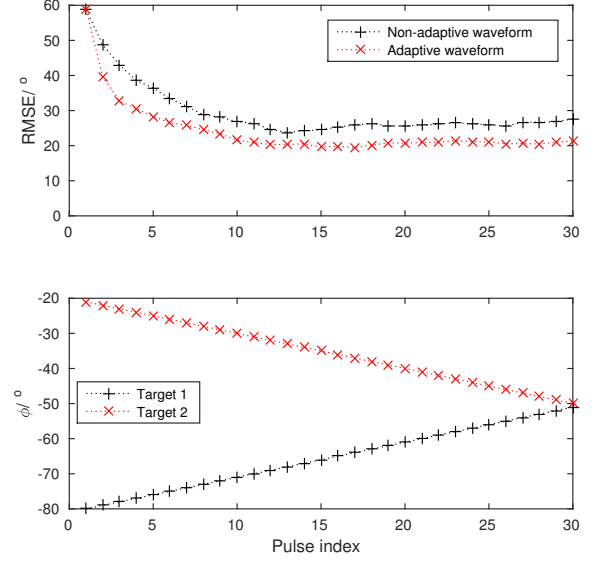
Fig. 2. RMSE and target motion for scenario 2
