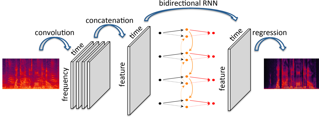
Fig. 1: Model architecture. EHNET consists of three components: noisy spectrogram is first convolved with kernels to form feature maps, which are then concatenated to form a 2D feature map. The 2D feature map is further transformed by a bidirectional RNN along the time dimension. The last component is a fully-connected network to predict the spectrogram frame-by-frame. EHNET can be trained end-to-end by defining a loss function between the predicted spectrogram and the clean spectrogram.
