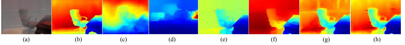
Fig. 3: Depth estimation results on (a) NYU synthetic dataset by methods (c) Chen et al. [4], (d) Karsch et al. [7], (e) He et al. [5], (f) Berman et al. [1], (g) Chen et al. [3] and (h) ours, compared with (b) ground truth. The PM2.5 value estimated by our method is 208.402 \mu\text{g}/\text{m}^3 .
