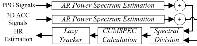
Fig. 1. Overall block diagram for the proposed method
