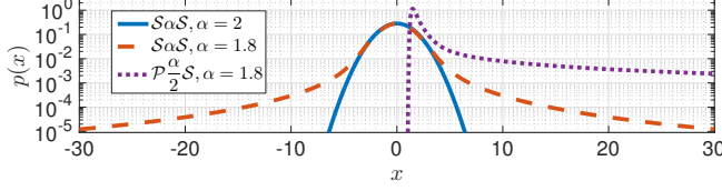
Fig. 1. Approximately computed pdfs of S_\alpha S_c and P_{\frac{\alpha}{2}} S for x \in \mathbb{R} .
