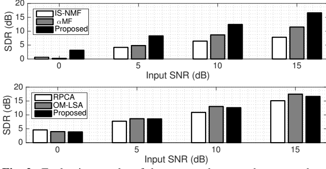
Fig. 2. Evaluation results of the proposed approach on speech enhancement. Top: comparison with semi-supervised methods, bottom: comparison with OM-LSA and RPCA.
