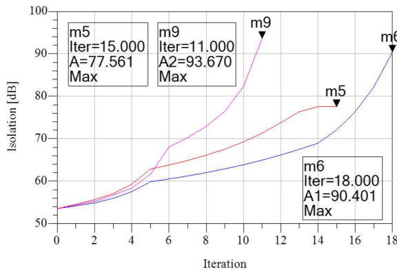
Fig. 4. Tuning of analog SI cancellation.
