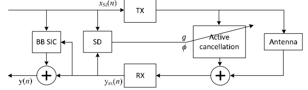
Fig. 2. Tuning of the active cancellation and baseband SI cancellation.
