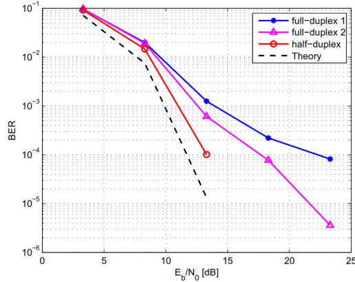
Fig. 5. BER results.
