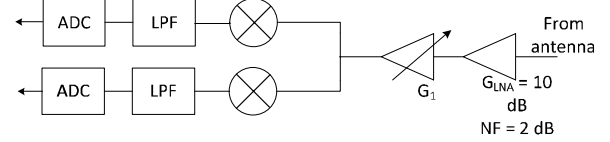
Fig. 3. Direct conversion receiver.
