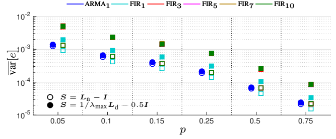
Fig. 2. Average empirical variance among all nodes of the error between the sparsified filter output and the original graph output for different values of p .
