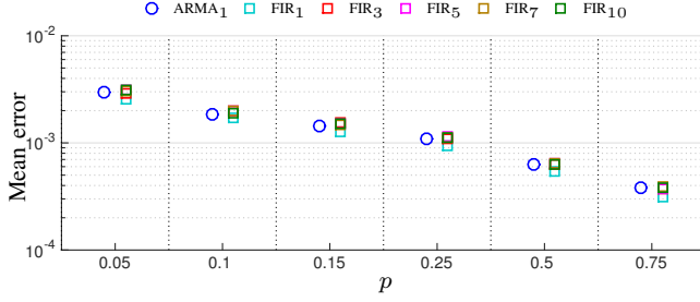
Fig. 1. Mean error over all nodes and realizations between deterministic and sparsified output for different values of p when \mathbf{S} = \mathbf{L}_n - \mathbf{I} .
