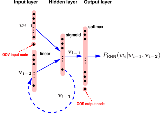
Fig. 1. A full output layer RNNLM with OOS nodes.
