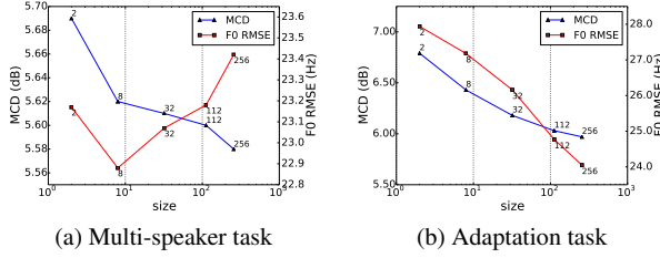
Fig. 3. Objective evaluation of different discriminant code sizes.
