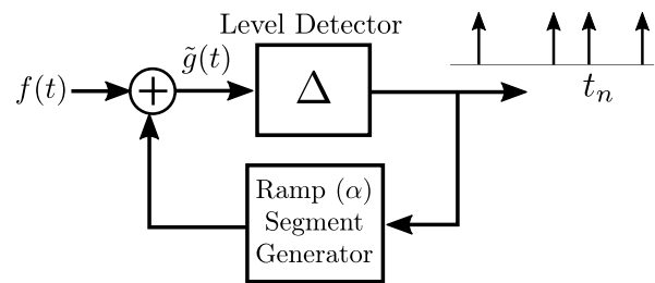
Fig. 1. Block-diagram representation.
