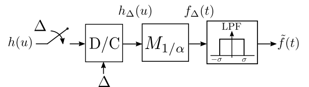
Fig. 2. Approximate reconstruction procedure for a bandlimited source signal f such that h = M_\alpha f . The block D/C is a discrete-to-continuous operation involving sinc interpolation with period \Delta .
