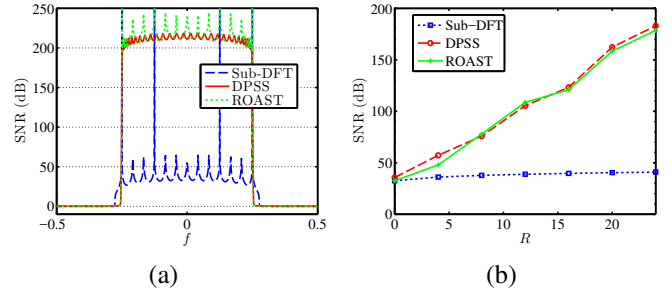
Fig. 1. (a) SNR captured by different projections for pure sinusoids e_f with R = 4 \log(N) ; (b) SNR captured by different projections for a sampled bandlimited signal \mathbf{x} with R ranging from 0 to 4 \log(N) . Here N = 1024 , W = \frac{1}{4} .
