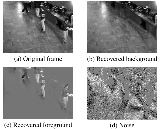
Fig. 3. SRPCP background and foreground recovery.
