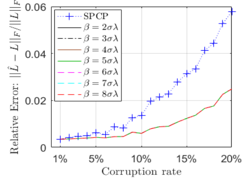
Fig. 2. Average Relative Error of \hat{\mathbf{L}} .
