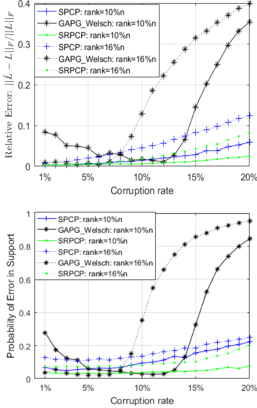
Fig. 1. Average Relative Error of \hat{\mathbf{L}} (top) and Probability of Error in Support (bottom).
