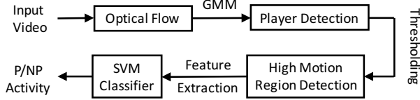
Fig. 2. Video analysis for P/NP activity detection.
