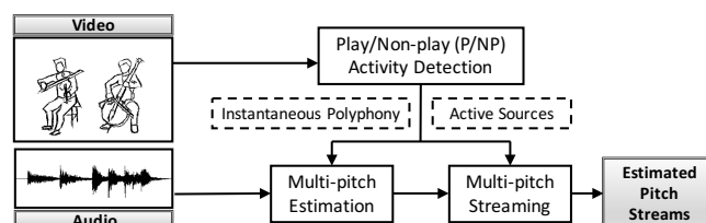
Fig. 1. Proposed framework for enhancing multi-pitch analysis using video-based play/non-play activity detection.
