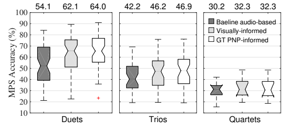
Fig. 5. Boxplot of MPS accuracy grouped by polyphony on all subsets derived from the 11 pieces, comparing the baseline audio-based method (dark gray), proposed visually informed method (light gray), and the incorporation of ground-truth PNP labels (white). The number above each box shows the mean value of the box.
