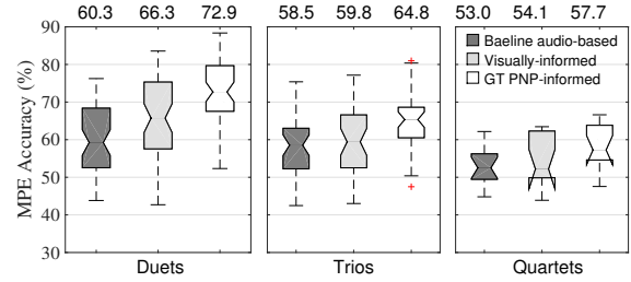
Fig. 4. Boxplot of MPE accuracy grouped by polyphony on all subsets derived from the 11 pieces, comparing the baseline audio-based method (dark gray), proposed visually informed method (light gray), and the incorporation of ground-truth PNP labels (white). The number above each box shows the mean value of the box.
