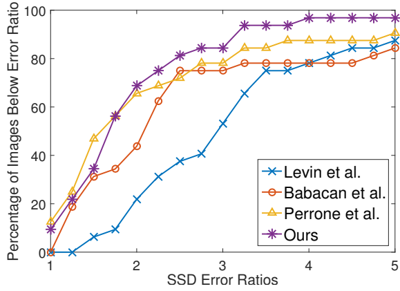
Fig. 1. Cumulative histogram of SSD error ratio
