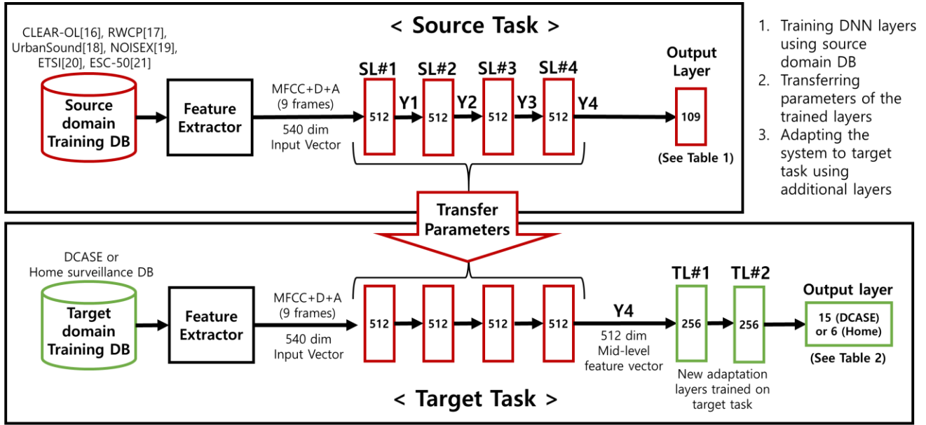
Fig. 1. Proposed transfer learning based DNN framework for acoustic scene classification
