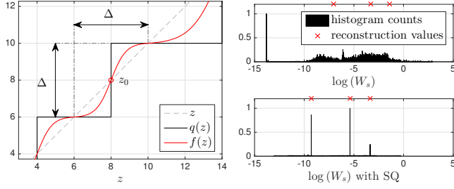
(a) Derivable approximation f(\cdot) of scalar quantization q(\cdot) . (b) Histograms of \log(W_s) for coder NTF without and with SQ.
