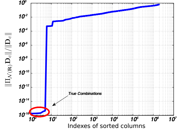
Fig. 2: Normalized functional (16) for the columns \tilde{\mathbf{D}} , in the noise free case, sorted in ascending order. In this example M = 9 and N = 5 .
