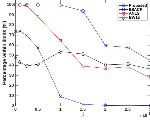
Fig. 2. Percentage of pitch estimates found within \pm 3\% of the ground truth in the simulated data case.
