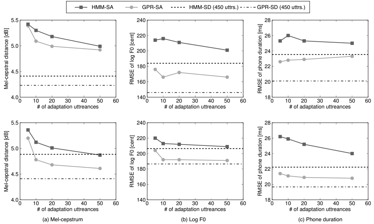
Figure 3: Acoustic feature distortions between original and synthetic speech. Upper and lower rows show the results of speaker MHT and MSH, respectively.
