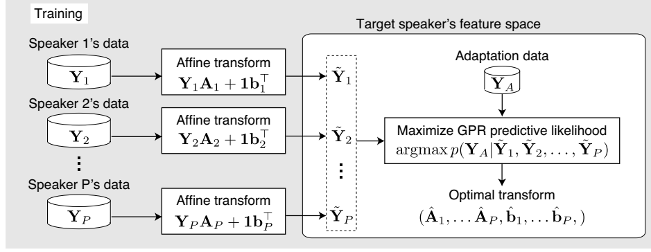
Figure 1: Outline of training of adaptation parameters.
