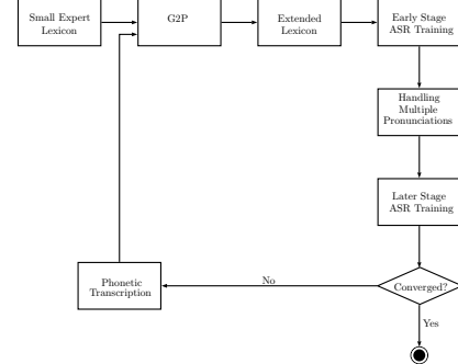
Fig. 1. An iterative framework for lexicon generation and acoustic modeling
