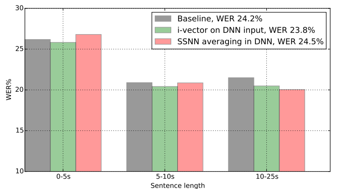
Fig. 2. Performance on dev set, subdivided by sentence lengths (complete recipe, sMBR systems from table 2). The i -vector inputs (estimated per-speaker) are helpful for all sentence lengths, while “summary vectors” (extracted per-sentence) are deleterious for short sentences and helpful for sentences longer than 10 seconds.
