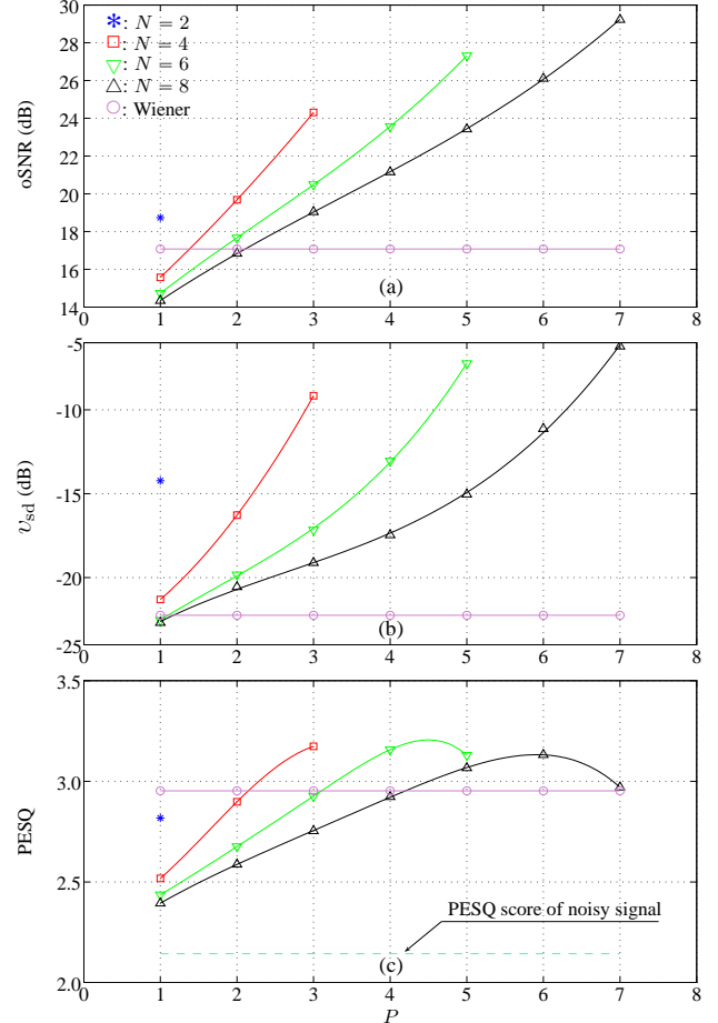
Fig. 1. Performance of \mathbf{h}_o(k, n) and the traditional Wiener filter in white noise as a function of P and N : (a) oSNR, (b) v_{sd} , and (c) PESQ score. The input SNR is 10 dB.
