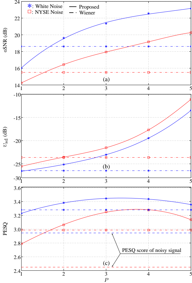
Fig. 2. Performance of \mathbf{h}_o(k, n) and the traditional Wiener filter in white and NYSE noises as a function of P : (a) \text{oSNR} , (b) v_{sd} , and (c) PESQ score. The input SNR is 10 dB and N = 6 .
