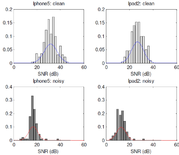
Fig. 1. SNR distribution for the clean and noisy environments on iPhone5 and iPad2.
