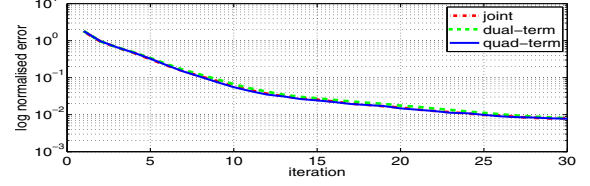
Fig. 2. Log normalised average error versus LBP iterations for the joint, dual-term and the quad-term separable likelihoods.
