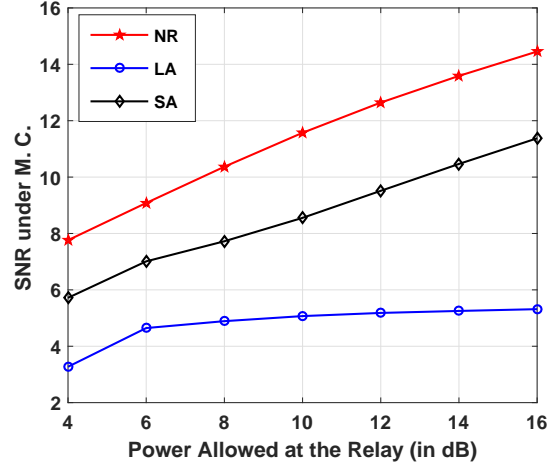
Fig. 1. SNR results for different schemes.
