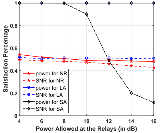
Fig. 2. Satisfaction probability of the constraints.
