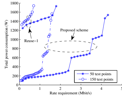
Fig. 2. A comparison of network power consumption between the proposed scheme and Reuse-1 scheme in [2].
