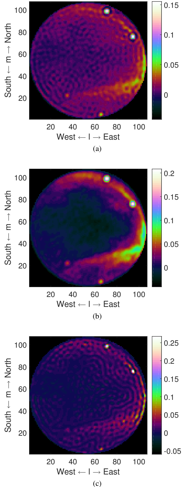
Fig. 2. Image estimates based on (a) truncated eigenvalue decomposition, (b) triangular-weighted eigenvalue decomposition, (c) dirty image based conditioning.
