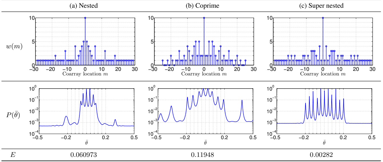
Fig. 2. Comparison among (a) nested arrays, (b) coprime arrays, and (c) super nested arrays in the presence of mutual coupling. The MUSIC spectra P(\bar{\theta}) are computed under 0dB SNR, 500 snapshots, 10 sensors, and D = 11 sources, as marked by ticks on the \bar{\theta} axis. The mutual coupling model (7) has c_1 = 0.5e^{j\pi/3} , c_\ell = c_1 e^{-j\pi(\ell-1)/8}/\ell , and B = 100 .
