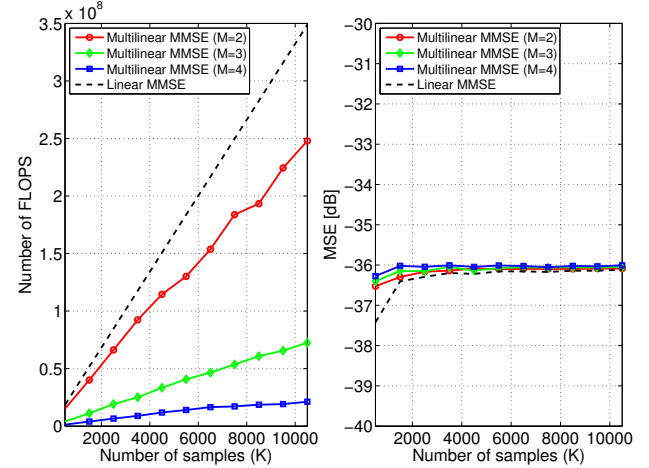
Fig. 3. Performance for a varying sample size for N = 128 sensors.
