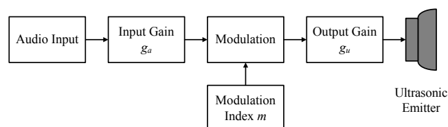
Fig. 1. An illustration of the parametric array loudspeaker.
