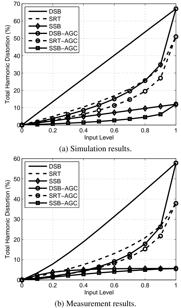
Fig. 3. Validation of the automatic gain control (AGC) for the PAL.
