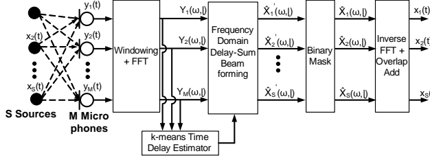
Fig. 1. Block diagram of our proposed algorithm.
