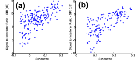
Fig. 4. SIR for time delays extracted from different frames versus the silhouette of the frame for two sources (a) Source B (b) Source C.
