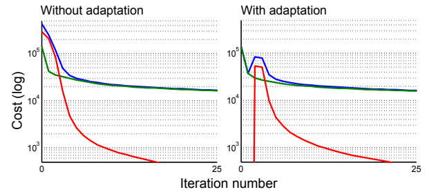
Fig. 3. Evolution of the reconstruction cost (in green), constraints cost (in red) and total cost (in blue) with (right graphic) and without (left graphic) the weight adaptation method, in function of the iteration number.
