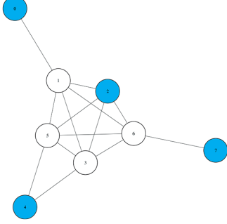
Fig. 2: Representing echo combinations as nodes in a graph. The set of blue nodes correspond to the (maximum) independent set.
