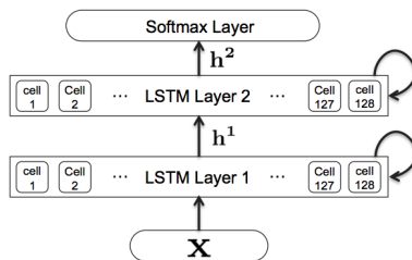
Fig. 1. LSTM architecture
