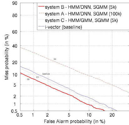
Fig. 1. DET curve – speaker verification results with scores pooled from five NIST SRE 2010 conditions (cond1 - cond5). We plot i-vector (baseline) and SGMM systems with different configurations as described in Section 5.2.1.
