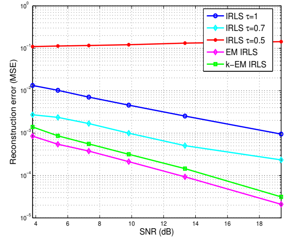
Fig. 3. Mean square error after 40 iterations as a function of the SNR for classical IRLS (with \tau = 1, \tau = 0.7 and \tau = 0.5 ) and the proposed EM-based algorithms.
