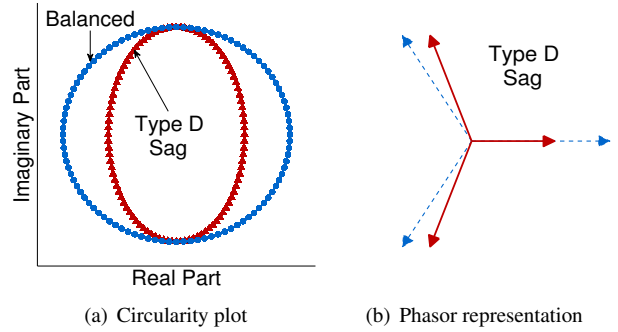
Fig. 2: Geometric and phasor diagrams for a Type D imbalance (voltage sag) of the three-phase power system voltages.
