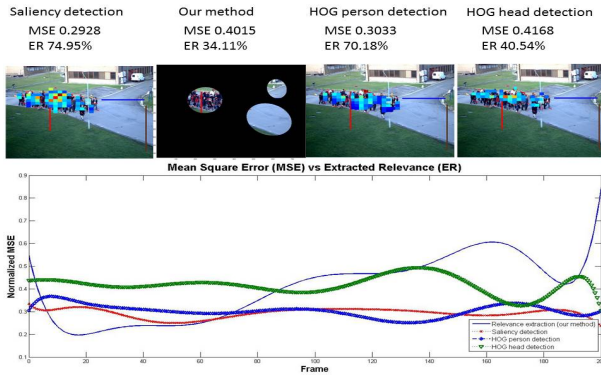
Fig. 5: Reconstruction comparison for different saliency extraction methods: saliency detection presented in [14]; HOG descriptors [15] combined with a learning-based SVM classifier for person (pedestrian) and head detections. The average mean square error normalized to 1 and the percentage of the crowd density map average acquired from the system (i.e. Extracted Relevance-ER) are shown.
