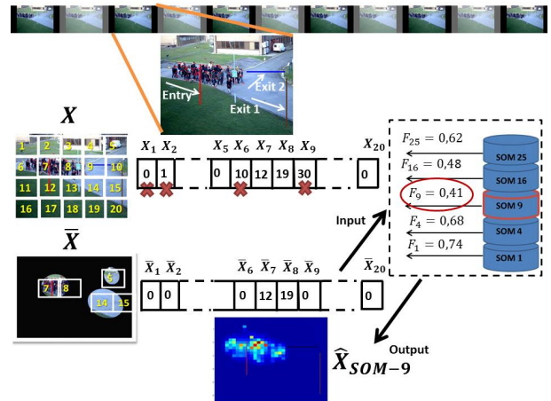
Fig. 3: Salient information extraction and crowding density map reconstruction
