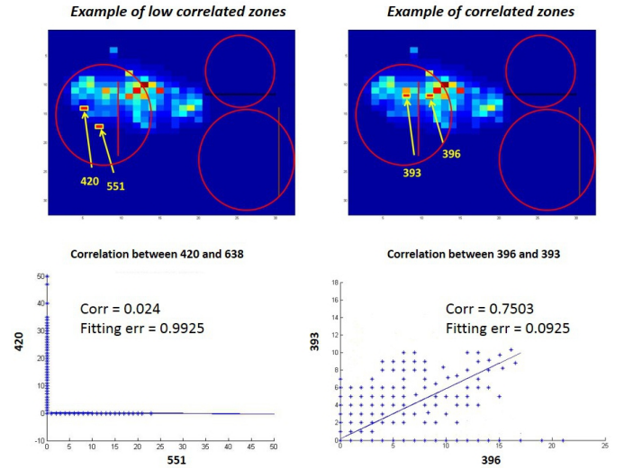
Fig. 2: Example of correlations analysis between locations pairs. The data are represented by the number of feature extracted by Lucas-Kanade optical flow associated to each cell
