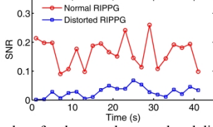
Fig. 4. The SNR values for the sample normal and distorted RPPG waves.
