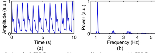
Fig. 3. A typical CPPG wave and its normalized spectrum: (a) CPPG wave, (b) Normalized spectrum.
