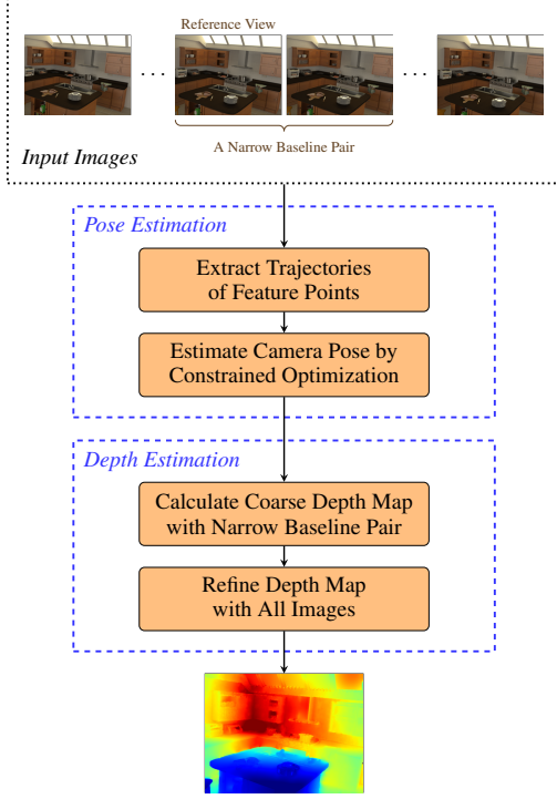
Fig. 2. Flowchart of the proposed depth estimation system: 1) Camera poses are first estimated from feature point trajectories under the constraint of linear translation. 2) Coarse depth map for the reference view is calculated from a narrow-baseline pair; then refined depth map is obtained using information from all views.
