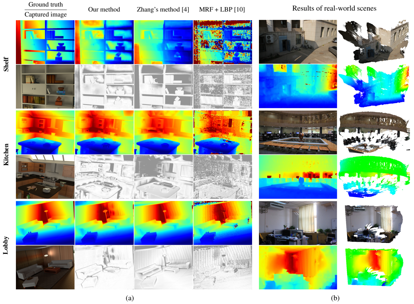
Fig. 6. (a) Results on the synthetic data set. Odd rows show the ground truth depth maps and those obtained by three different methods, while even rows show corresponding captured images and error maps of three different methods with respect to the ground truth. Darker areas in error maps mean larger errors. (b) Results of real-world scenes. Captured image, restored depth map and rendered point clouds (with two different coloring setups) are shown here.
