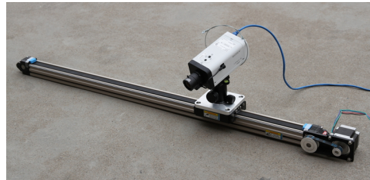
Fig. 1. The sliding camera system, in which a single camera on the track is controlled by a stepping motor.
