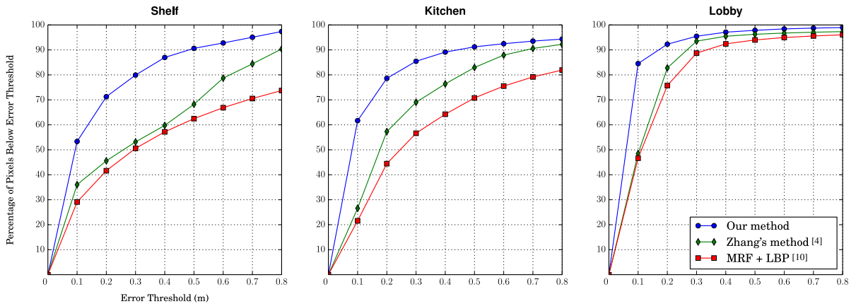
Fig. 7. Statistical comparison between different depth estimation methods on the synthetic data set. Our algorithm achieves higher accuracy than conventional methods.
