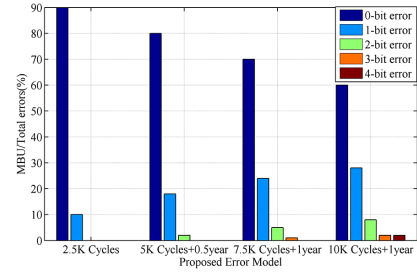
Fig. 5. Percentage of MBU errors in 4 proposed error models.
