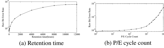
Fig. 1. RBER versus retention time and P/E cycle count for MLC devices.
