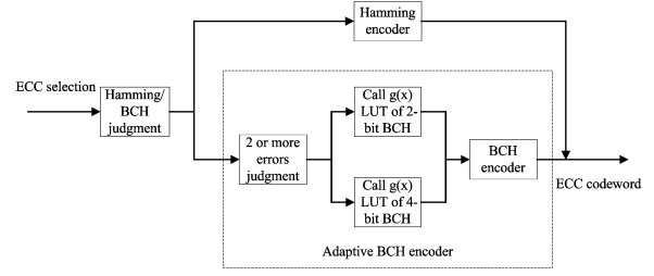
Fig. 3. Major steps in the adaptive ECC encoder.
