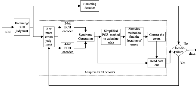
Fig. 4. Major steps in the adaptive ECC decoder.
