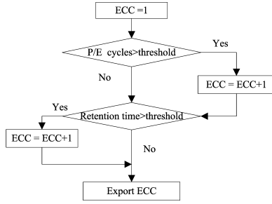
Fig. 2. Major steps in the determination of ECC.
