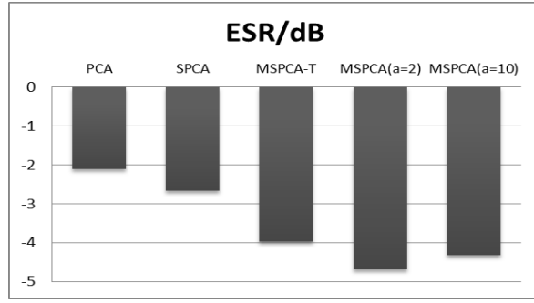
Fig. 3 Objective performance on extraction accuracy measured by ESR for PCA, SPCA, MSPCAs.
